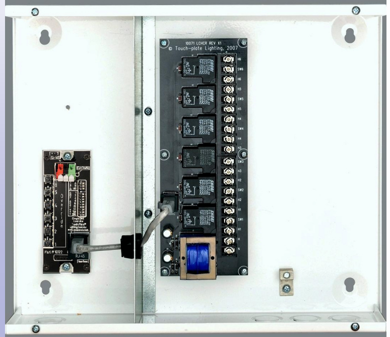
ZoneZ-SN-6RP Pictured above in New Enclosure
