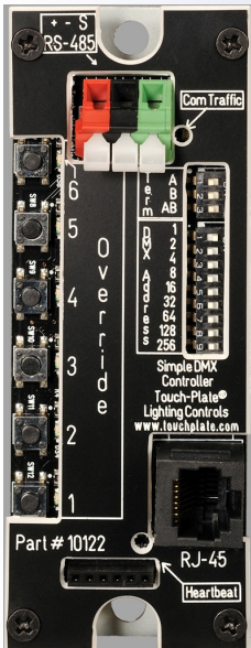
Model: Simple DMX Controller Board
