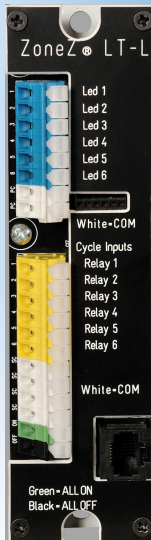
Model: 10116 Relay Control Board
