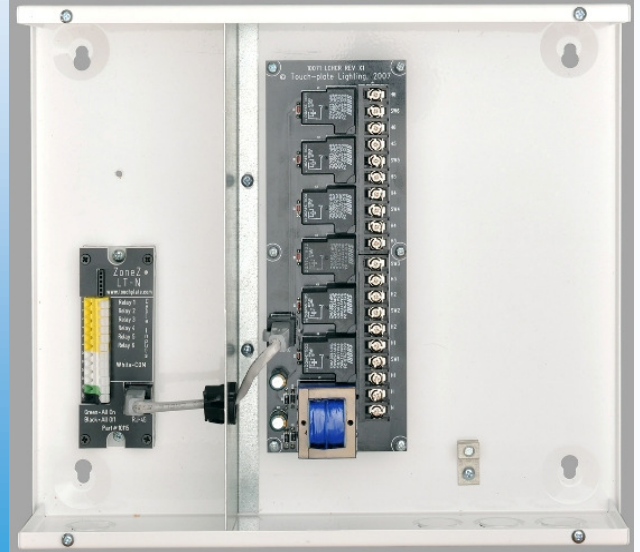
ZoneZ-LT-N-6RP Pictured Above in New Enclosure
