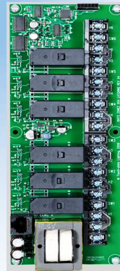
Model: 10071 Relay Board
