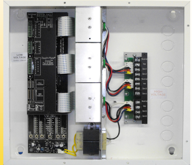
ZoneZ-D-6 Dimmer Module Pictured Above in New Enclosure
