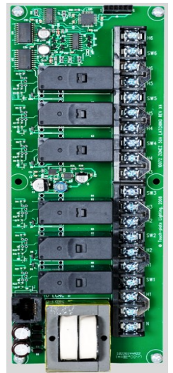
Model: 10072 Relay Board
