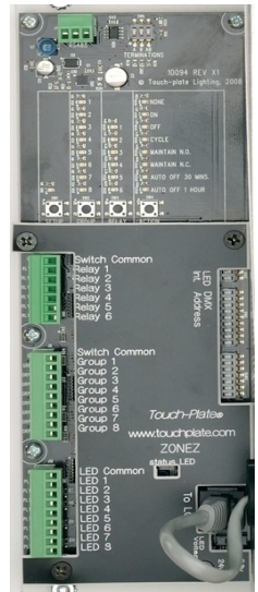
Model: 10094 Relay Control Board
