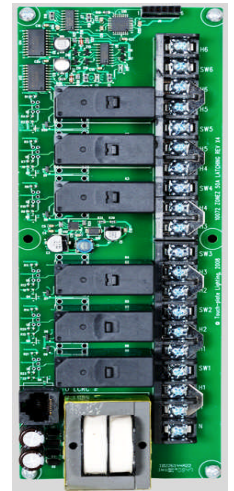
Model: 10072 Relay Board
